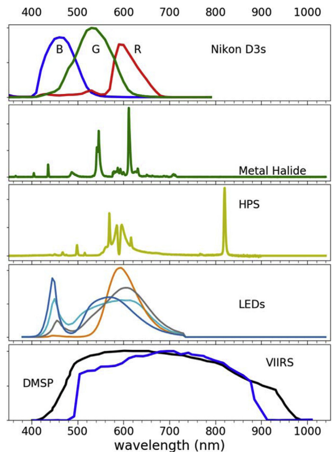
Fig. 24. Spectral response of the most popular sensors and most popular spectra, from top to bottom. (a) the spectral response of the Nikon D3s Cameras used by the astronauts at the ISS; (b) a typical spectra of a Metal Halide lamp, popular on architectural lights; (c) a High pressure sodium light, popular until 2014 on streelighting; (d) LEDs of 5000K (blue), 4000K (cyan), 2700K (grey) and PC-Amber(amber), popular on street lighting; (e) representative spectral response of DMSP/OLS(black) and SNPP/VIIRS/DNB(blue). Sources: Sánchez de Miguel (2015), Tapia Ayuga et al., (2015), Sánchez de Miguel et al., (2017), Elvidge, et al., 1999a,b,c and Liao et al., 2013. (For interpretation of the references to color in this figure legend, the reader is referred to the Web version of this article.)
